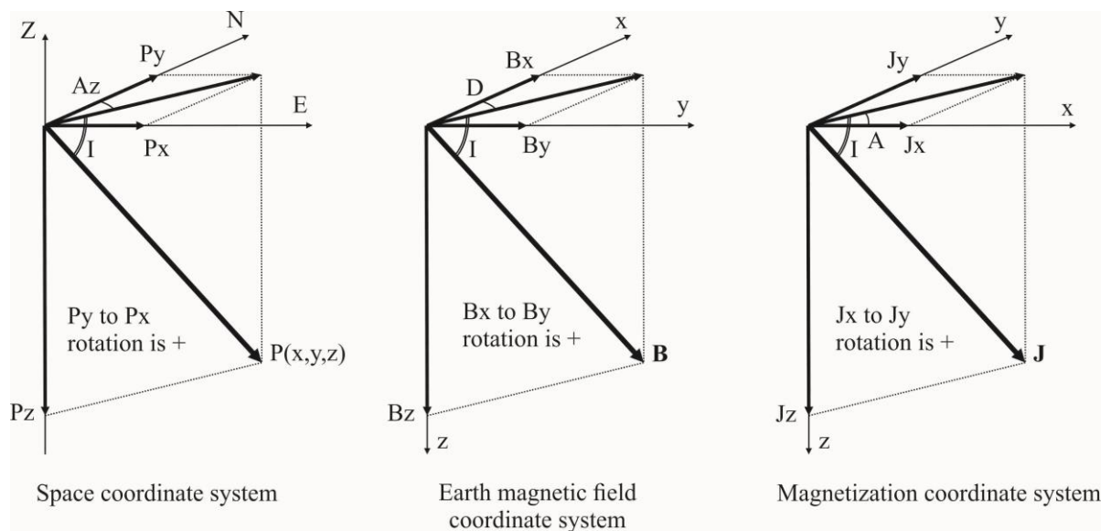
Figure 1.1 Magnetic parameters coordinate system
